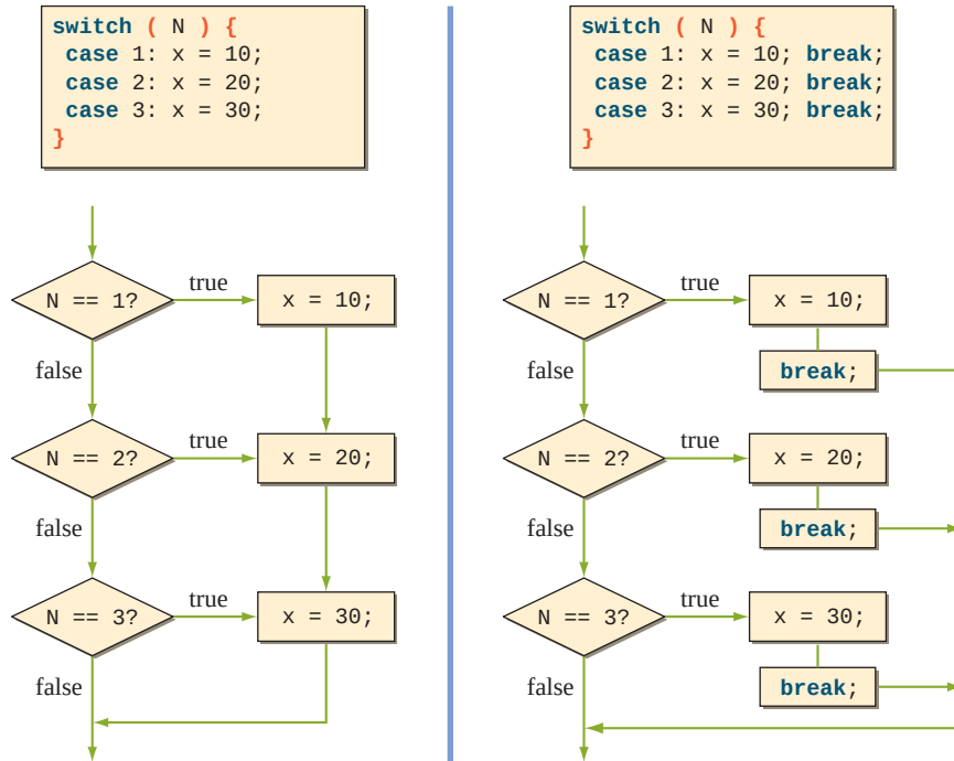
Figure 5.8 A diagram showing the control flow of the switch statement with and without the break statements.
