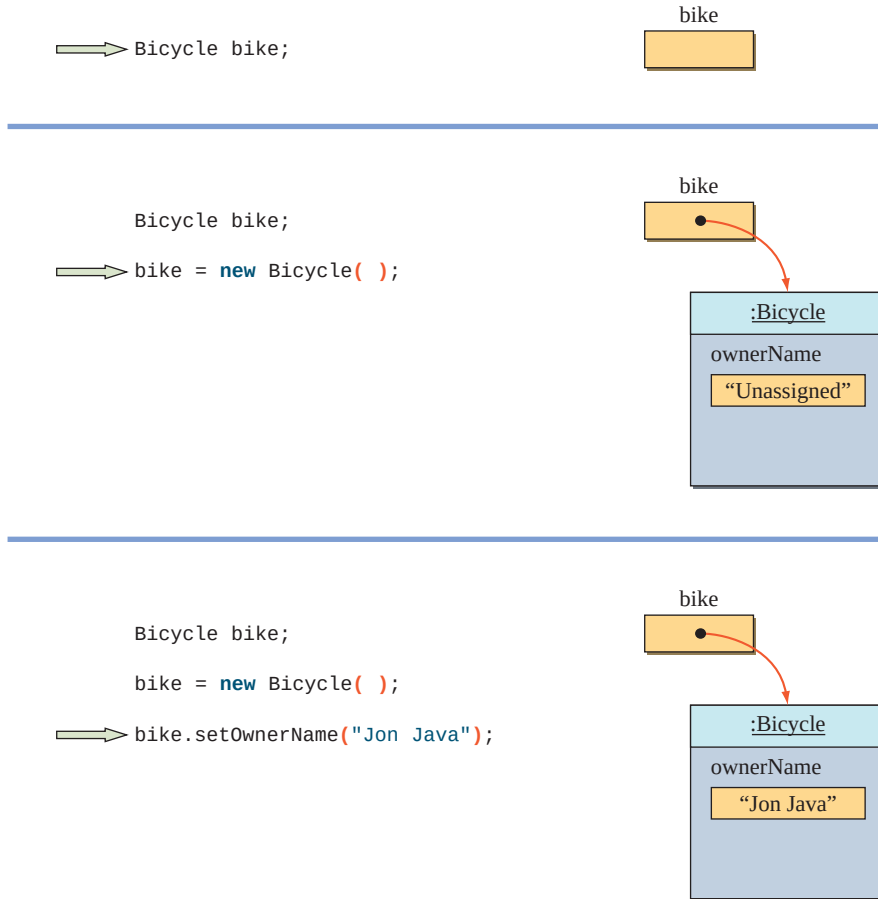
Figure 4.1 A sequence of state-of-memory diagrams that illustrate the effects of executing the constructor and the setOwnerName method of the Bicycle class.
