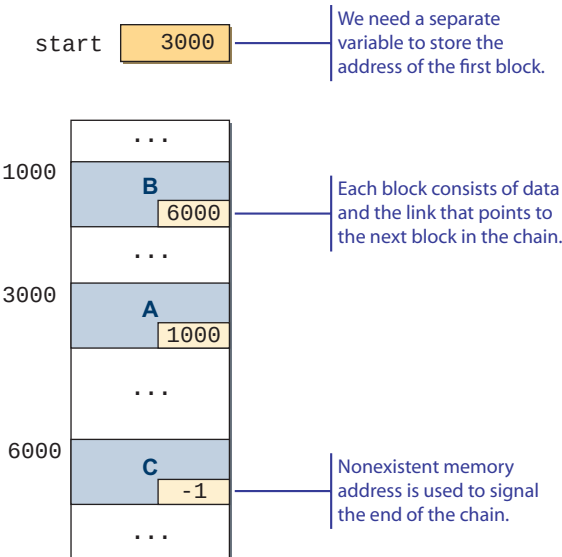
Figure 16.5 Three separate blocks of memory are allocated, with each block containing the address of the next block in the chain. Following the links from start , we visit blocks in the order of A, B, and C.
