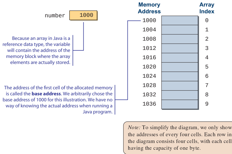
Figure 16.3 This diagram illustrates the contiguous memory allocation for an array of int.
