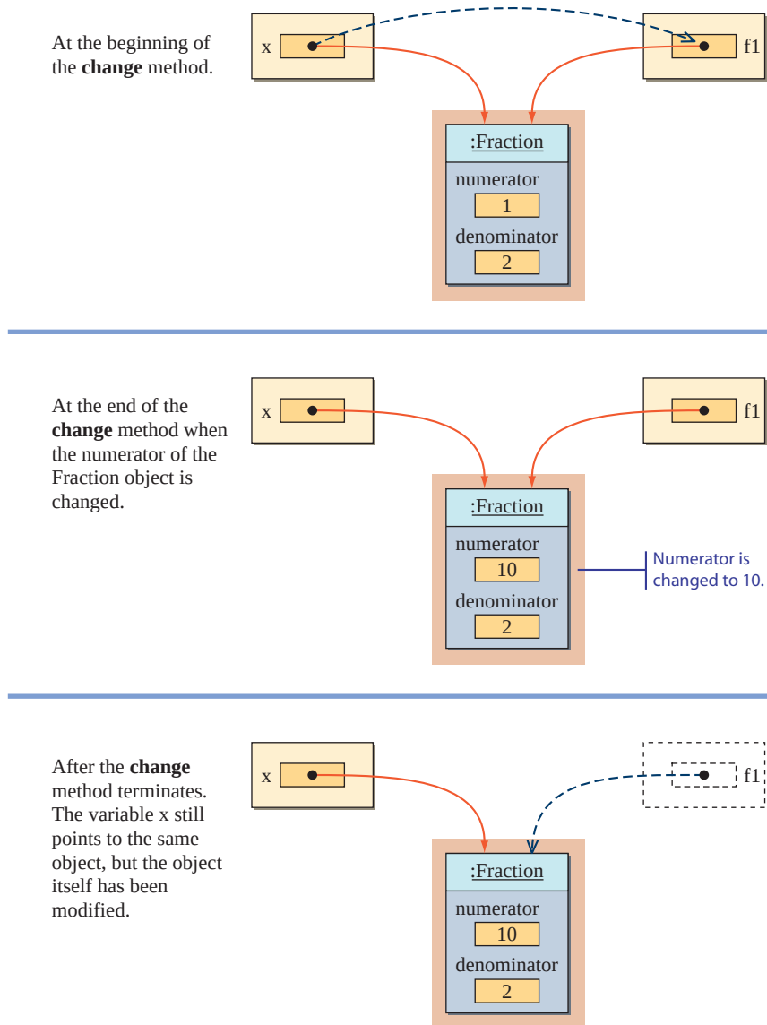
Figure 7.8 This illustration shows the effect of calling the change method.
