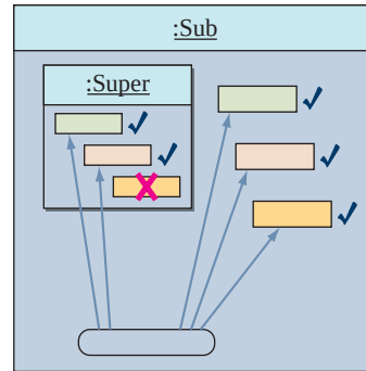
Figure 13.5 The difference between public , private , and protected modifiers. Everything except the private members of the Super class is visible from a method of the Sub class.
