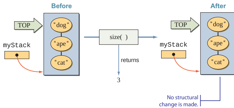
Figure 19.6 A sample size operation on the myStack stack.
