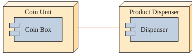
Figure 9 Deployment diagram.
