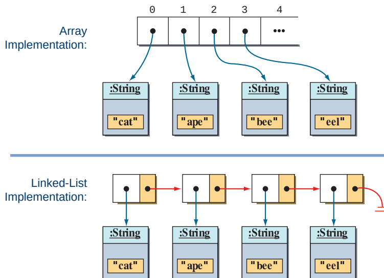
Figure 18.13 The structural difference between the array and linked-list implementations.
