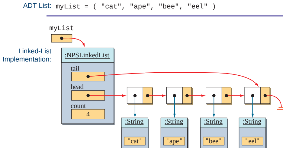
Figure 18.12 A linked-list implementation of the list myList .
