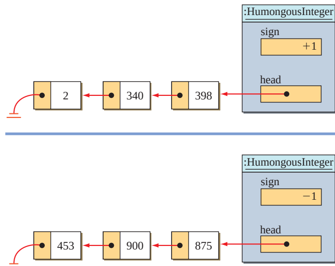
Figure 16.14 The diagrams illustrate the internal data structure for HumongousInteger objects. The top one represents 2340398 and the bottom one -453900875 .
