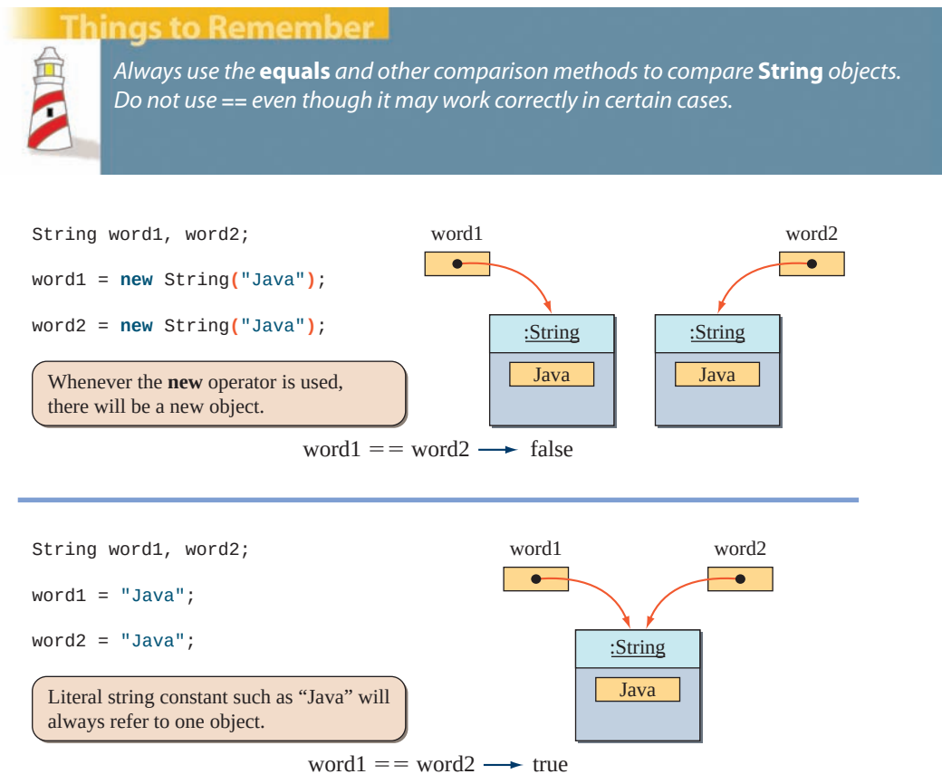
Figure 5.6 Difference between using and not using the new operator for String .
