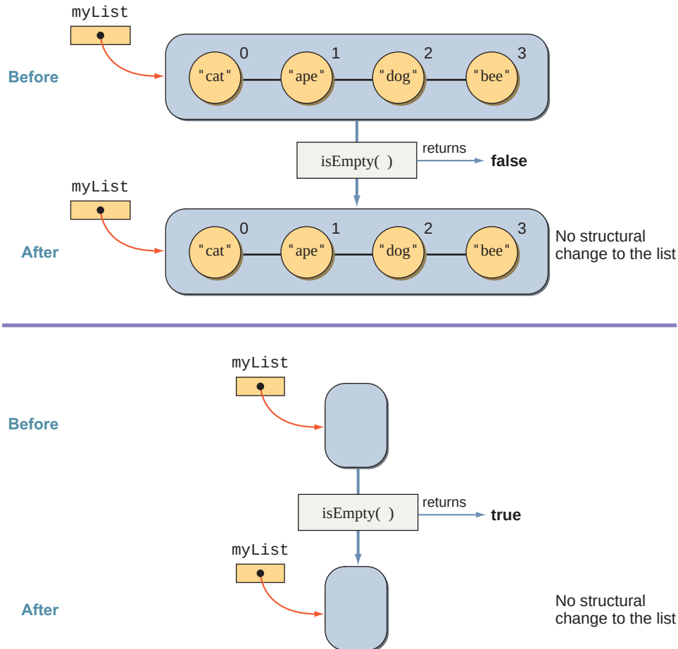
Figure 18.7 Sample isEmpty operations on the myList list.
