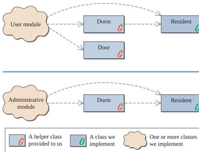
Figure 8.8 Program diagrams for the user and administrative modules. Notice the same Dorm and Resident classes are used in both programs. User and administrative modules will include one or more classes (at least one is programmer-defined).
