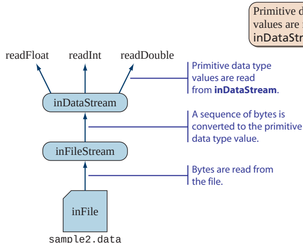
Figure 12.6 A diagram showing how the three objects inFile , inFileStream , and inDataStream are related.
