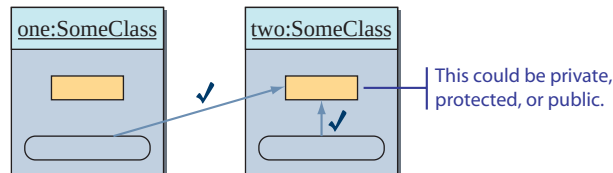
Figure 13.6 Data members accessible from an instance are also accessible from other instances of the same class.
