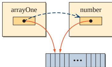
Figure 10.9 Passing an array to a method means we are passing a reference to an array. We are not passing the whole array.
