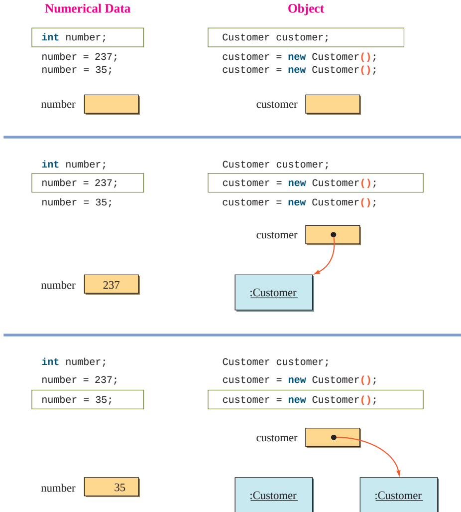
Figure 3.2 A difference between object declaration and numerical data declaration.
