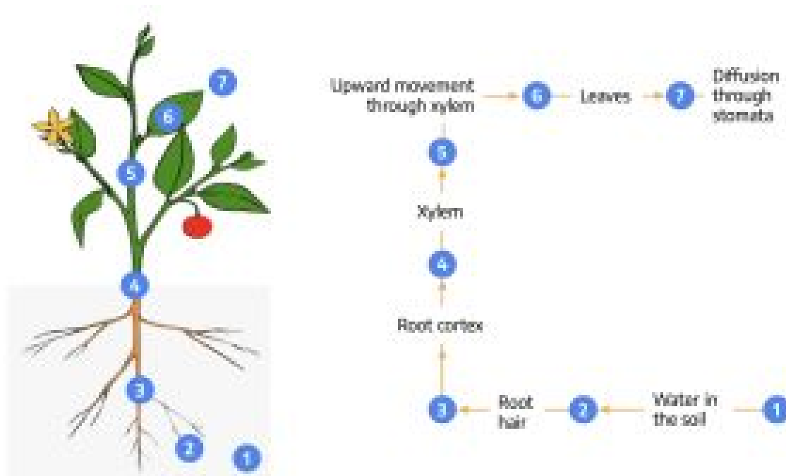
Diagram of evapotranspiration. Sheng-Yang He. CC BY-SA 4.0
