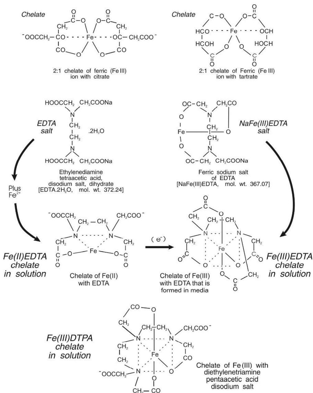
Fig. 3.6 Chemical structures of some chelating agents and iron chelates.
