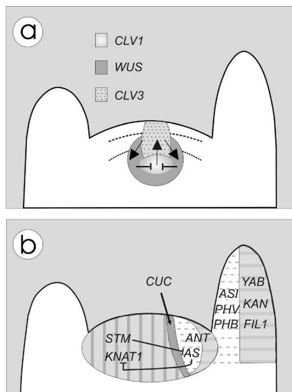
Fig. 8.4 – Genetic interactions in the shoot apical meristem. a: maintenance of the stem cells through the WUS/CLV auto-feed back loop; b: expression domains of selected genes involved in the establishment and patterning of leaf founder cells - for details of the genes noted in the figure, see Table 8.1 (adapted from Bowman and Eshed, 2000, by N. P  pin and E. Dubuisson, University P. M. Curie).
