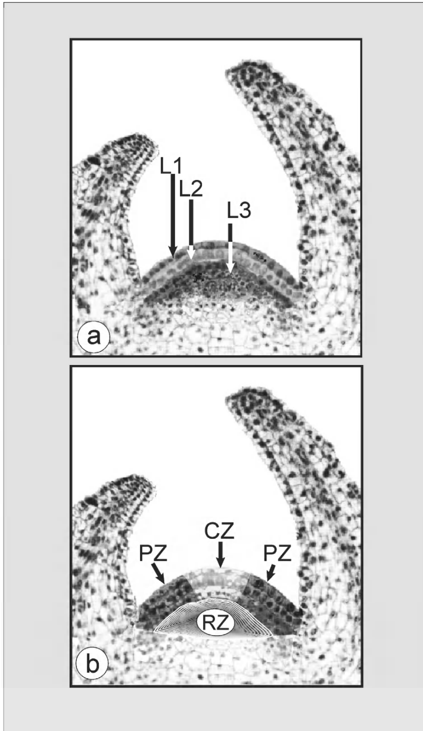
Fig. 8.2 – Layered (a) and zonated (b) structure of a tobacco vegetative shoot apical meristem. L1 –L3: layers; CZ: central zone; PZ: peripheral zone; RZ: rib zone (adapted from Bowman and Eshed, 2000, by N. Pépin, University P. M. Curie).
