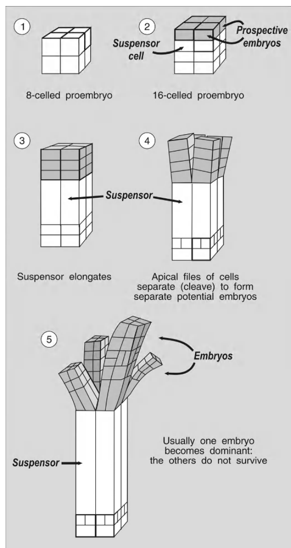
Fig. 10.7 A diagrammatic representation of zygotic cleavage embryogenesis in Pinus .
