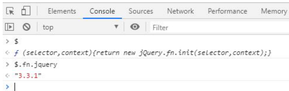
Figure 6-2. JavaScript library globals
