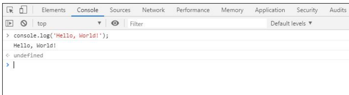
Figure 3-2. JavaScript example
