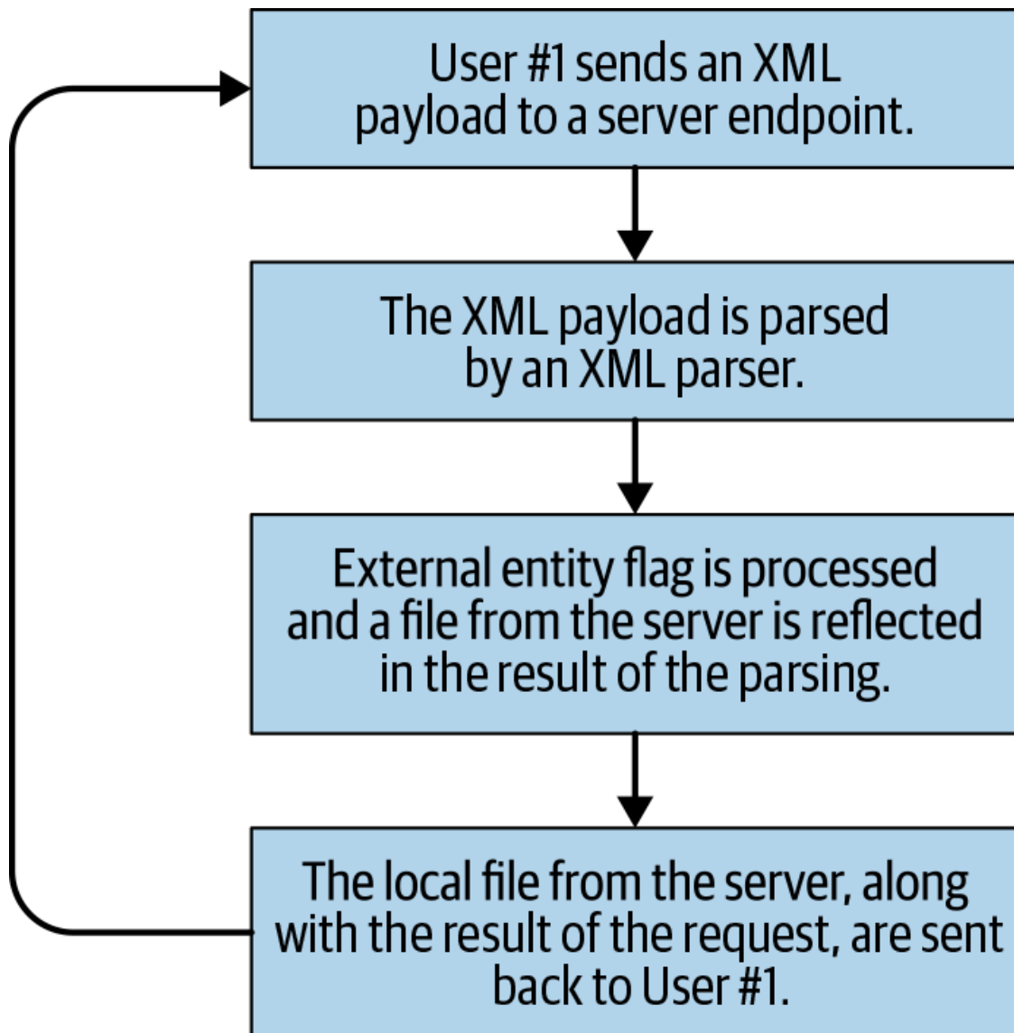
Figure 12-1. Direct XXE
