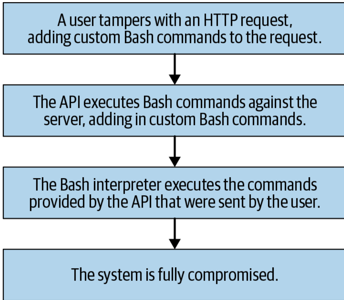
Figure 13-3. Command injection
