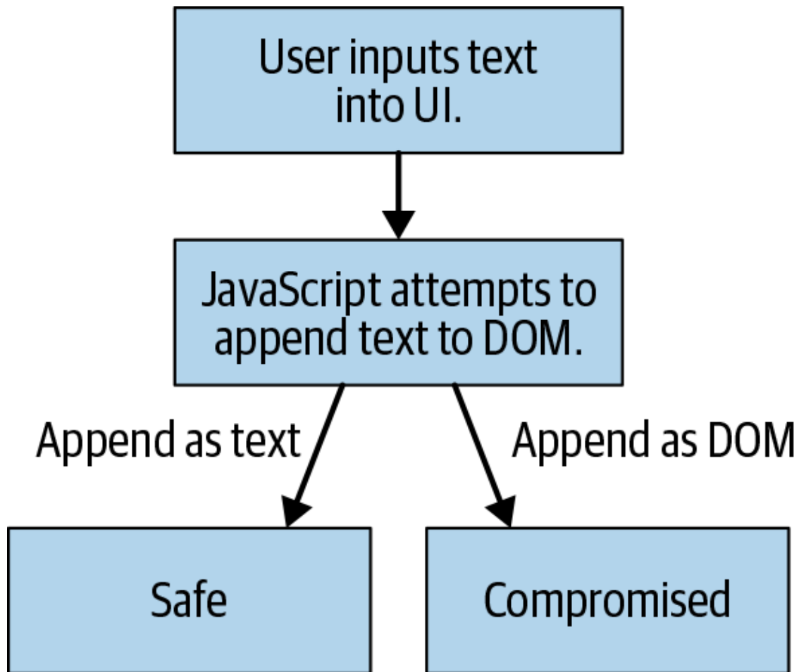
Figure 22-1. Most XSS (but not all) occurs as a result of user-supplied text being improperly injected into the DOM
