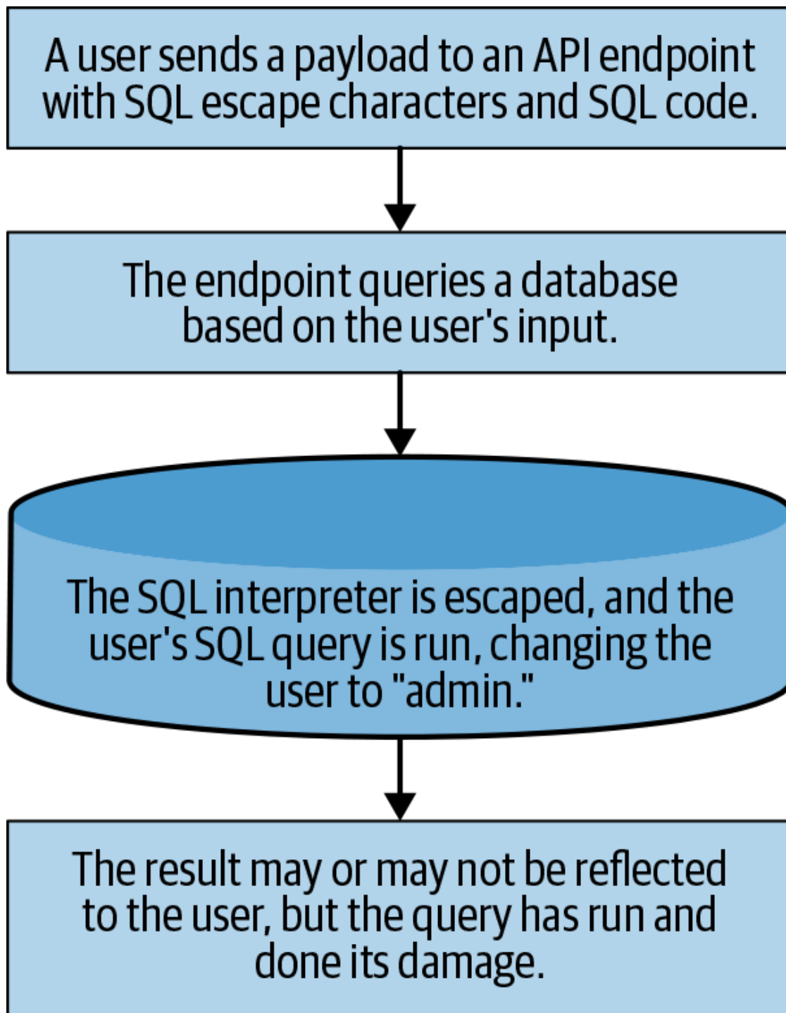
Figure 13-1. SQL injection
