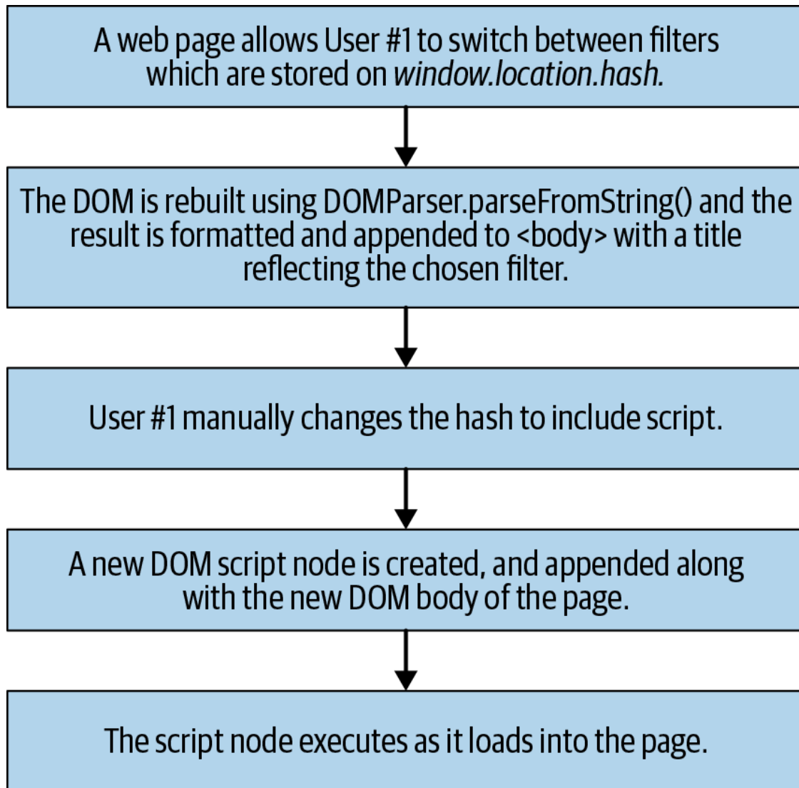
Figure 10-3. DOM-based XSS
