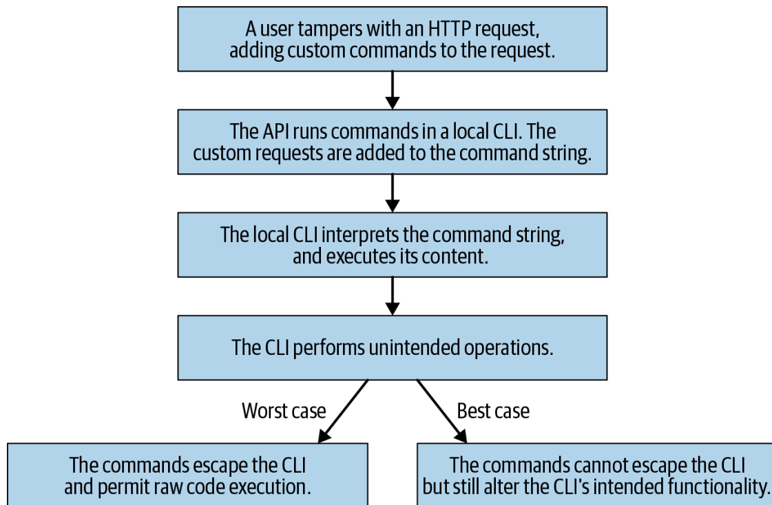
Figure 13-2. CLI injection
