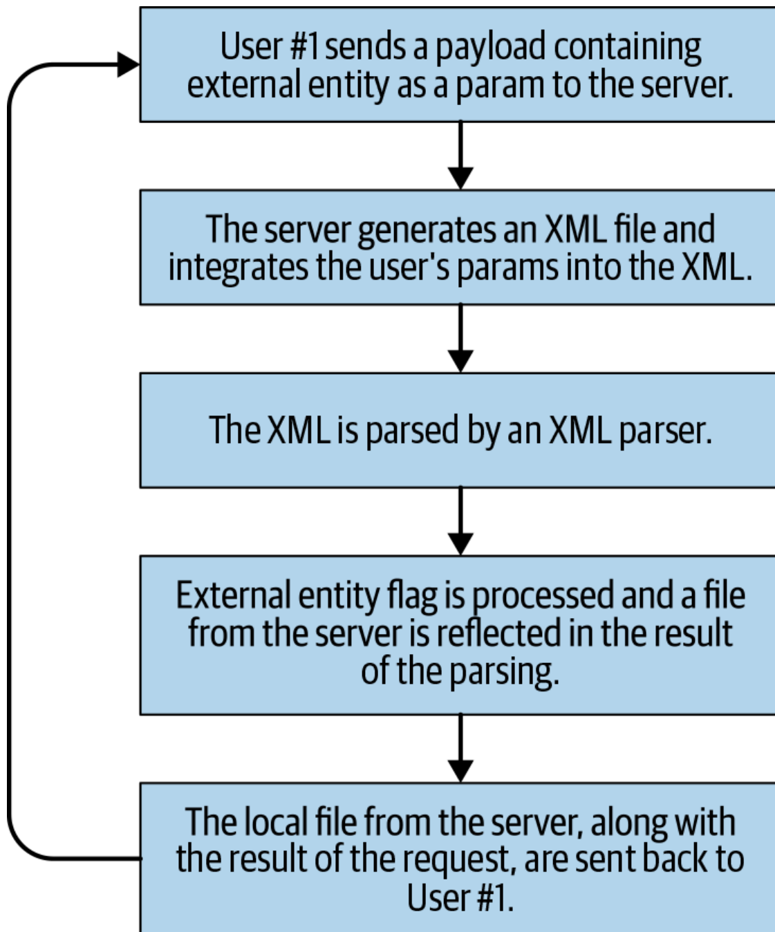
Figure 12-2. Indirect XXE
