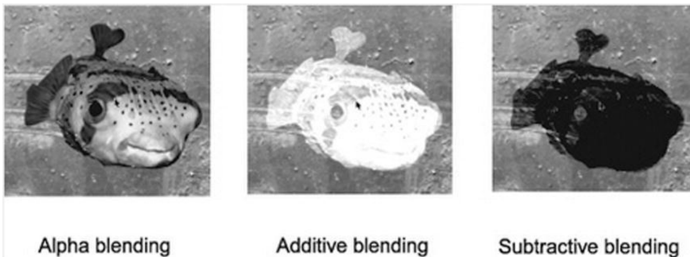
Figure 12-1. Blending effects
