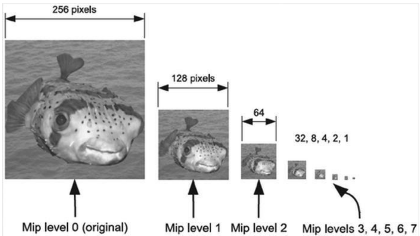
Figure 11-3. Mip maps
