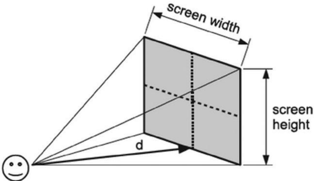
Figure 8-6. The viewing distance in a perspective projection
