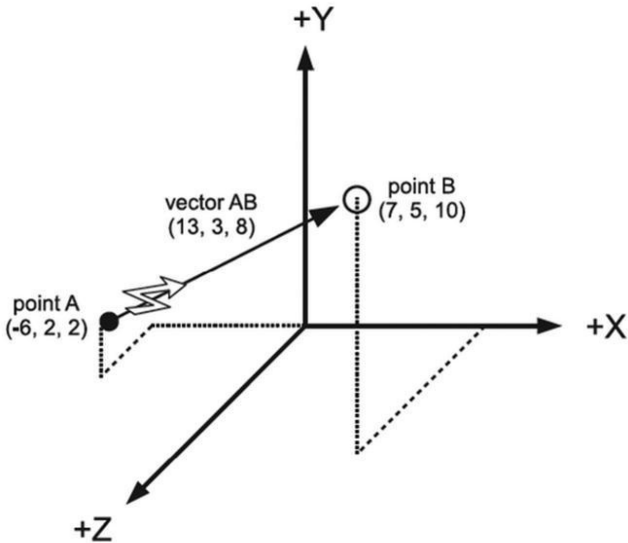
Figure 8-3. Calculating a target vector
