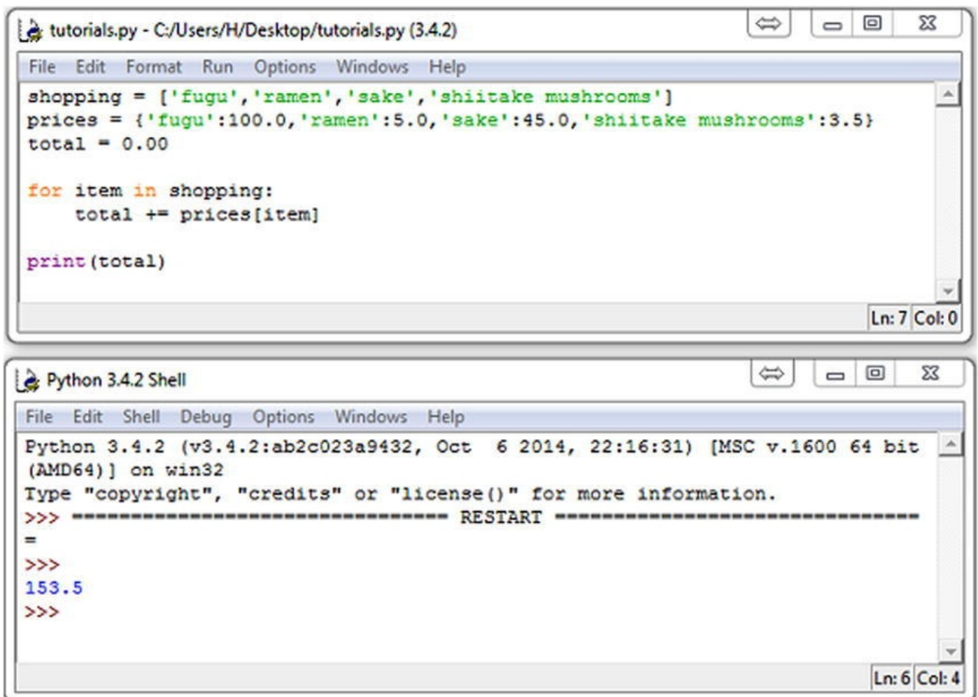
Figure 2-1. Python code in IDLE and the output console window
