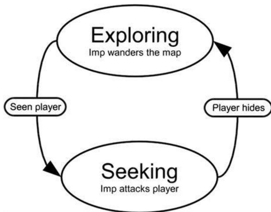
Figure 7-1. Imp state machine
