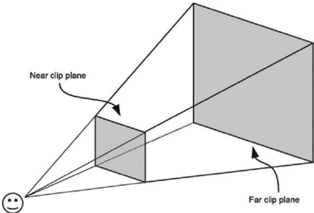
Figure 9-6. The viewing frustum
