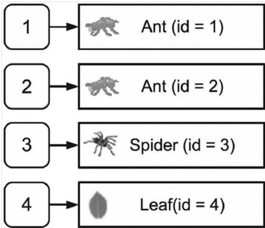
Figure 7-2. The entities dictionary
