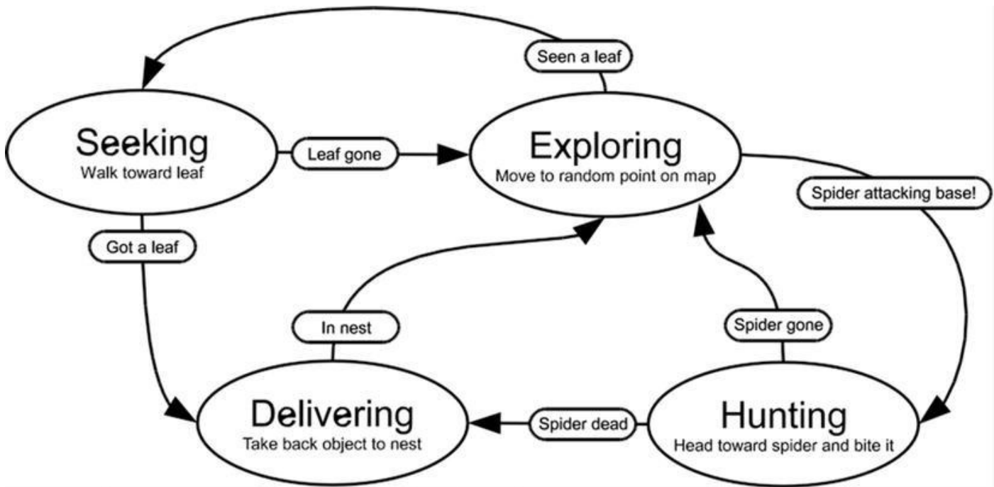
Figure 7-3. Ant state machine
