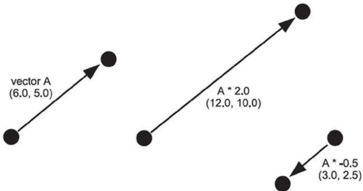
Figure 5-4. Multiplying a vector by a scalar
