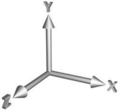
Figure 8-1. A three-dimensional coordinate system
