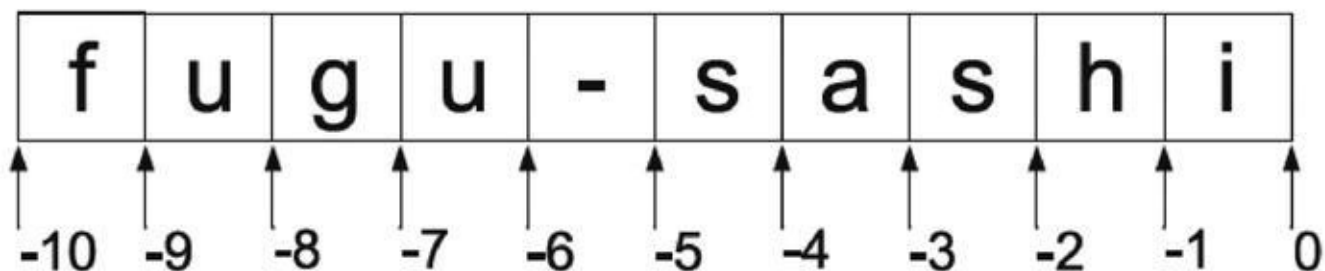
Figure 1-2. Negative indexing
