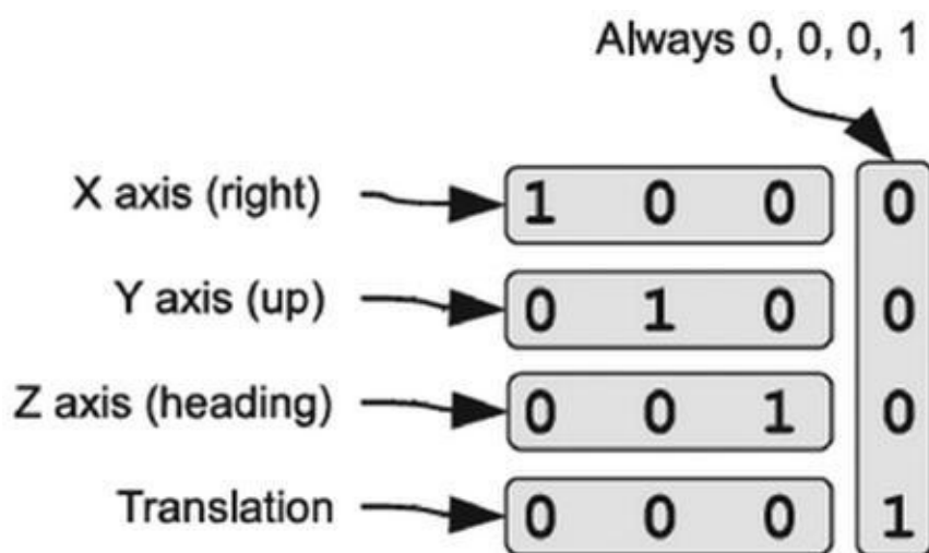
Figure 9-1. Components of a matrix
