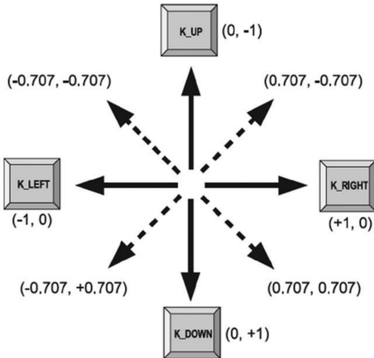
Figure 6-1. Diagonal vectors by combining simple vectors
