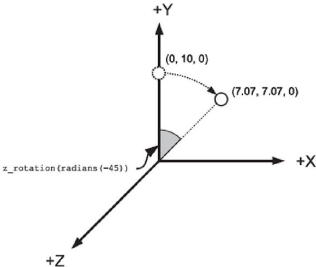
Figure 9-4. A rotation about the z axis
