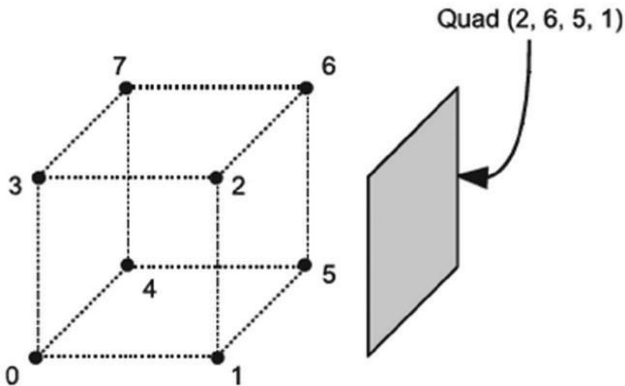
Figure 9-9. Faces and vertices
