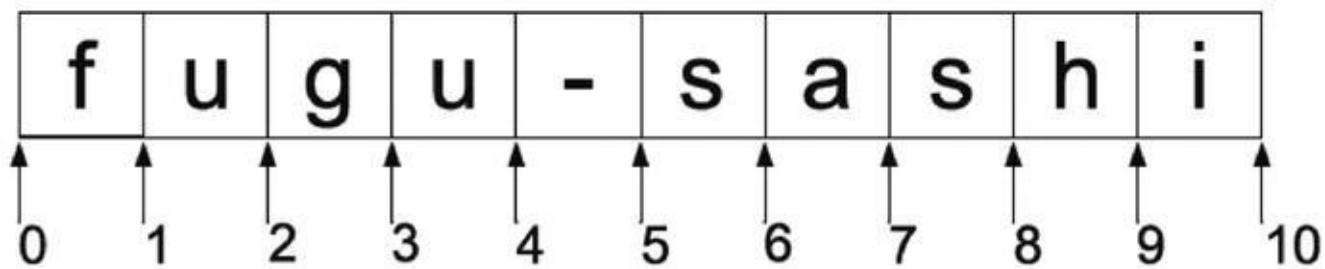
Figure 1-1. String indexing
