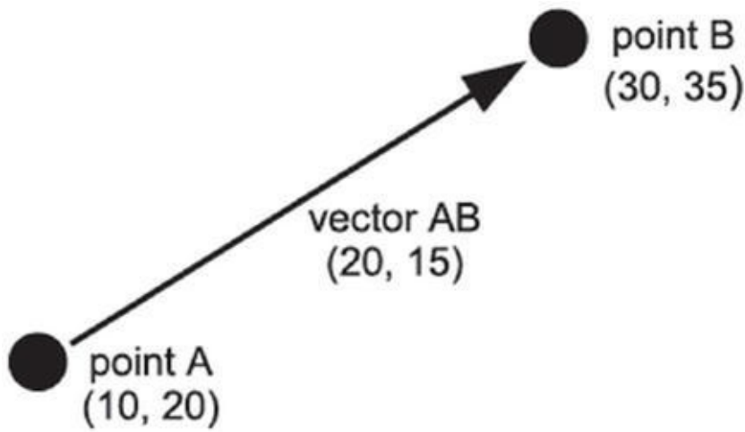
Figure 5-1. Creating a vector
