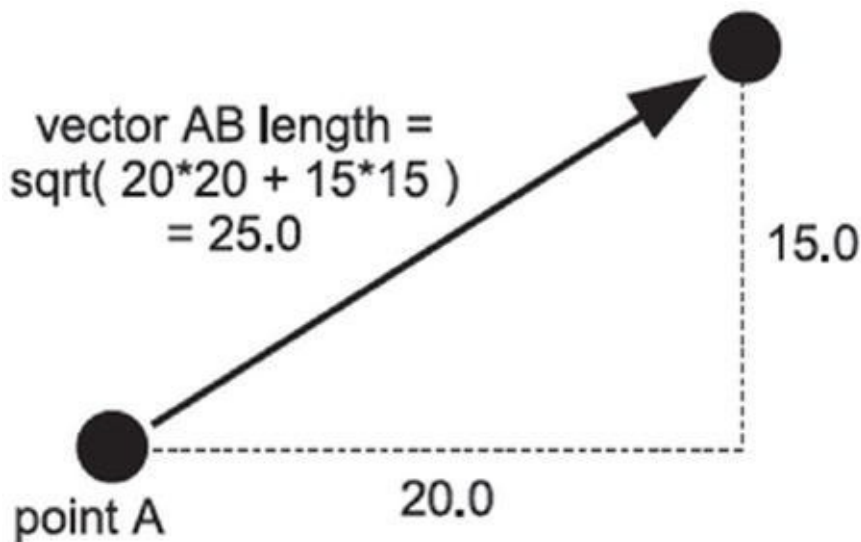
Figure 5-2. Creating a vector
