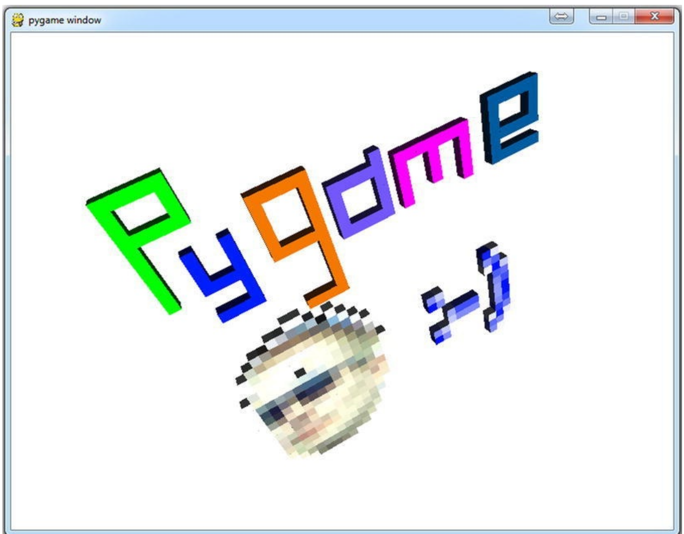
Figure 9-10. Cube world
