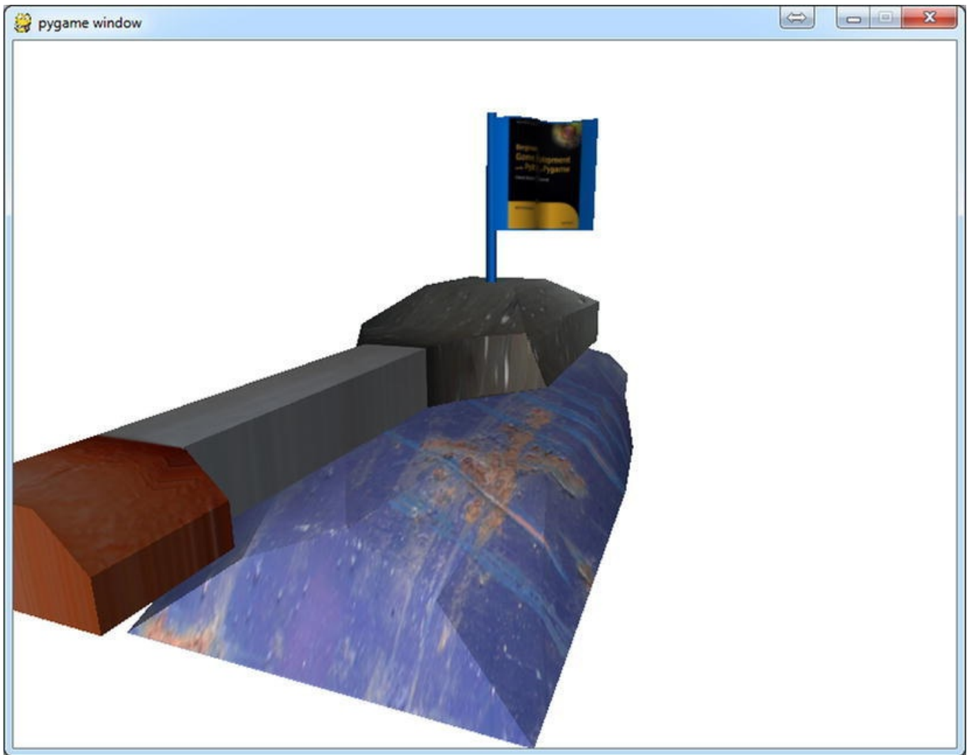
Figure 11-6. tankdemo.py
