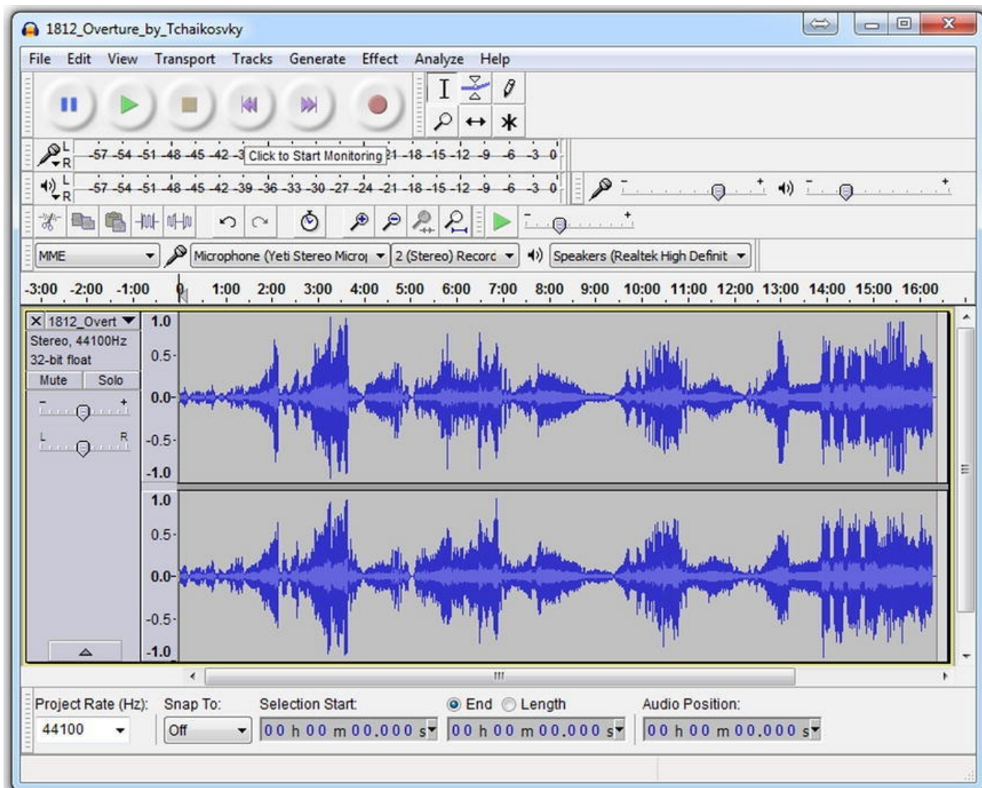
Figure 10-3. Audacity
