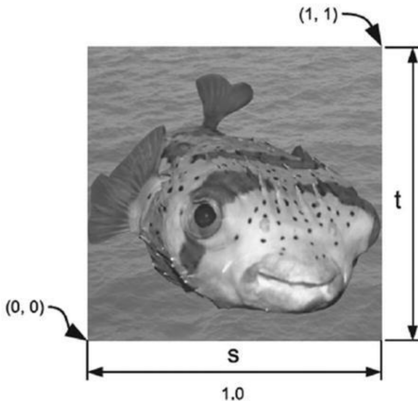
Figure 11-1. Texture coordinates
