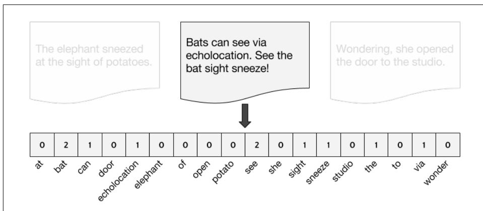
Figure 2-3. Token Frequency as Vector Encoding
