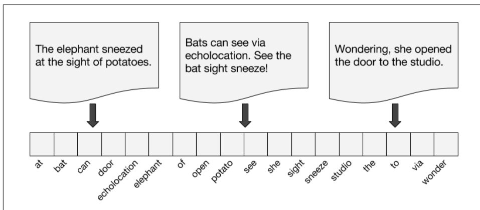
Figure 2-2. Encode Documents as Vectors
