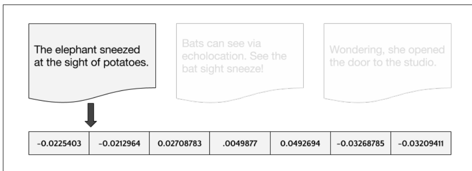
Figure 2-6. Distributed Representation
