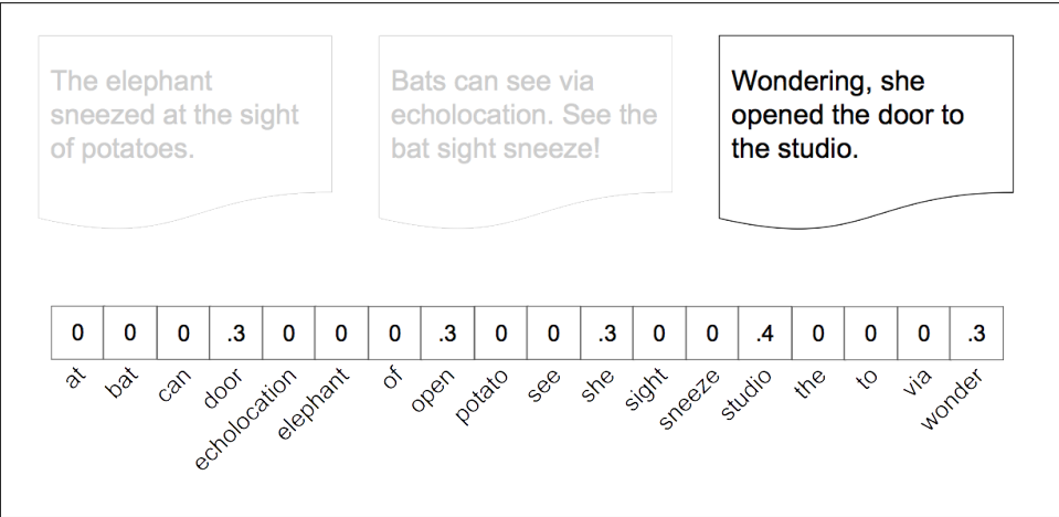
Figure 2-5. TF-IDF Encoding
