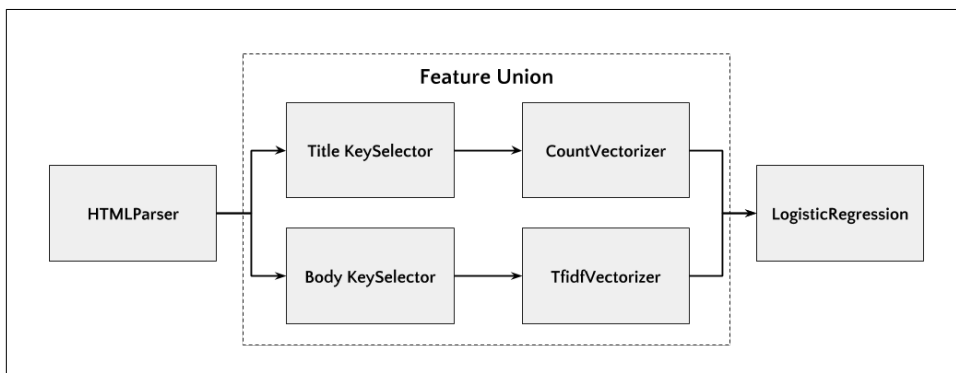
Figure 2-8. Feature Unions for Branching Vectorization
