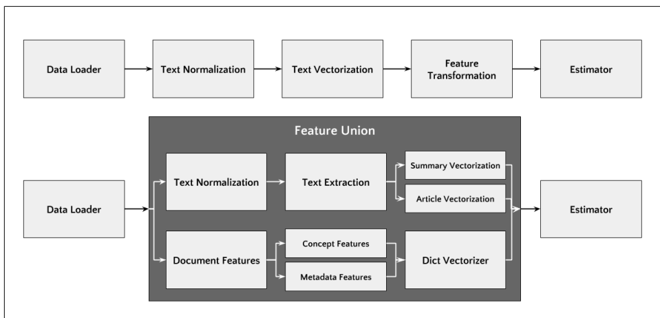
Figure 2-7. Pipelines for Text Vectorization and Feature Extraction
